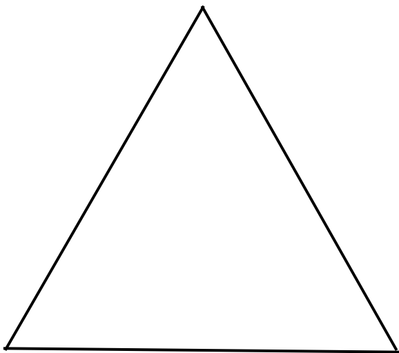
Equilateral Triangle
