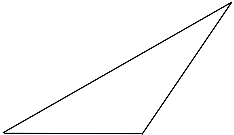
Obtuse Triangle
